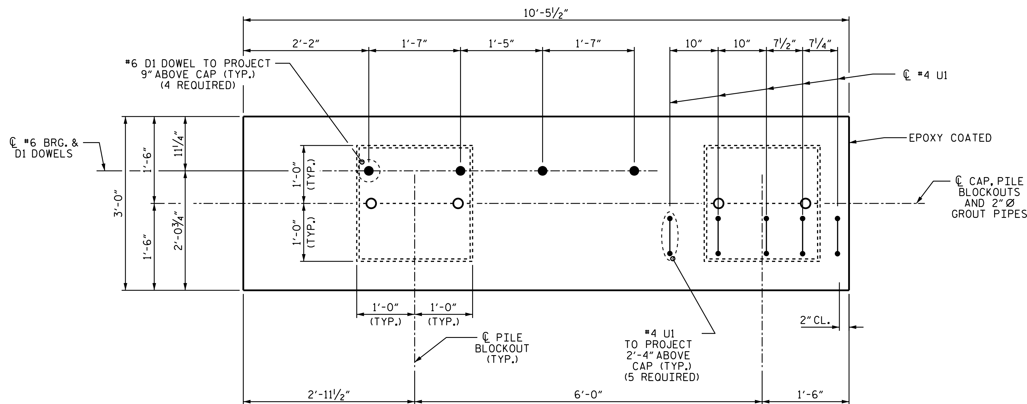
PLAN
