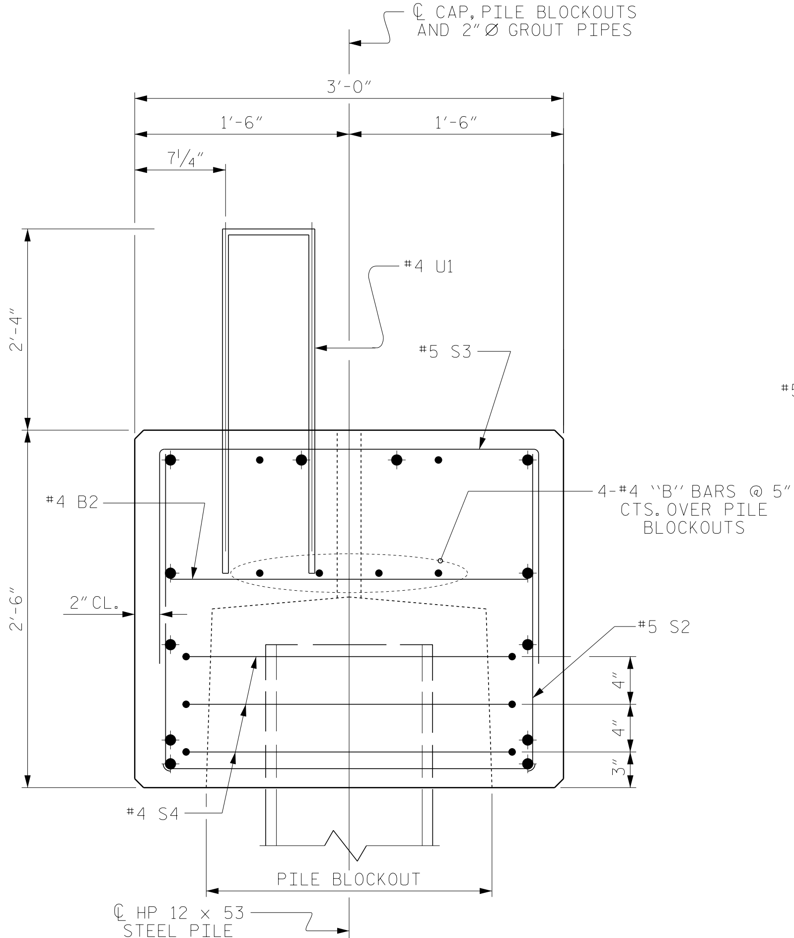
SECTION B-B
