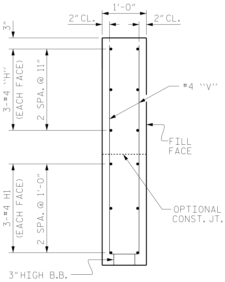
SECTION X-X
