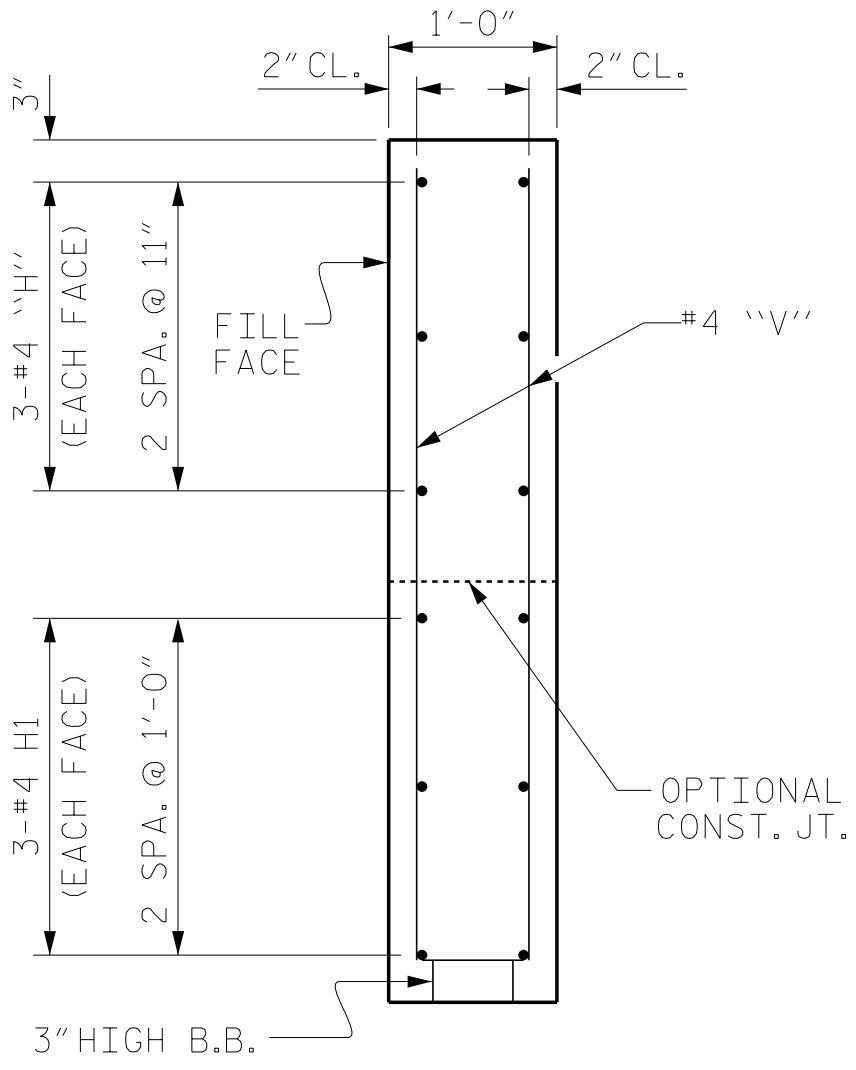
SECTION Y-Y
