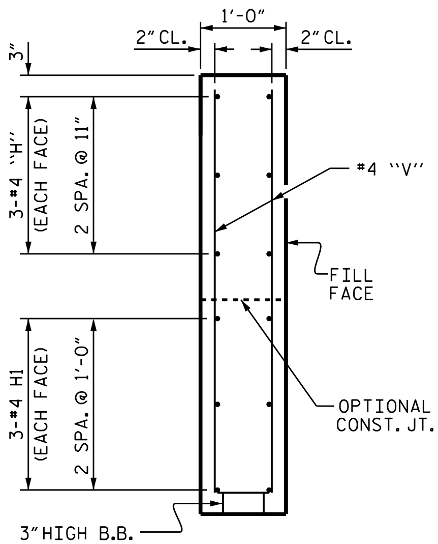
SECTION X-X
