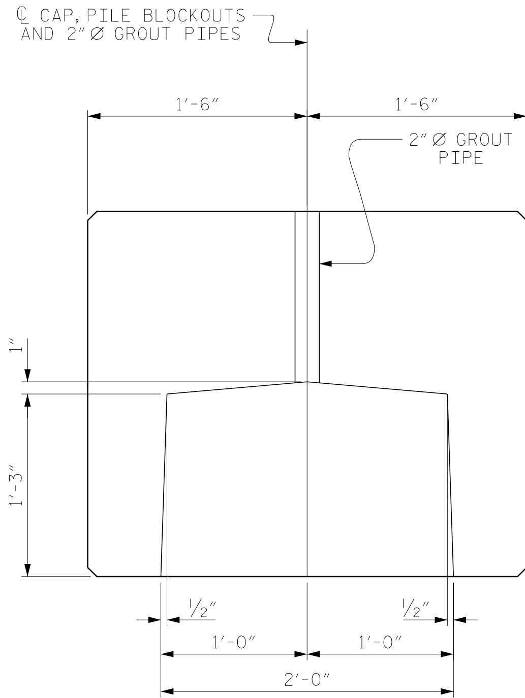
SECTION
