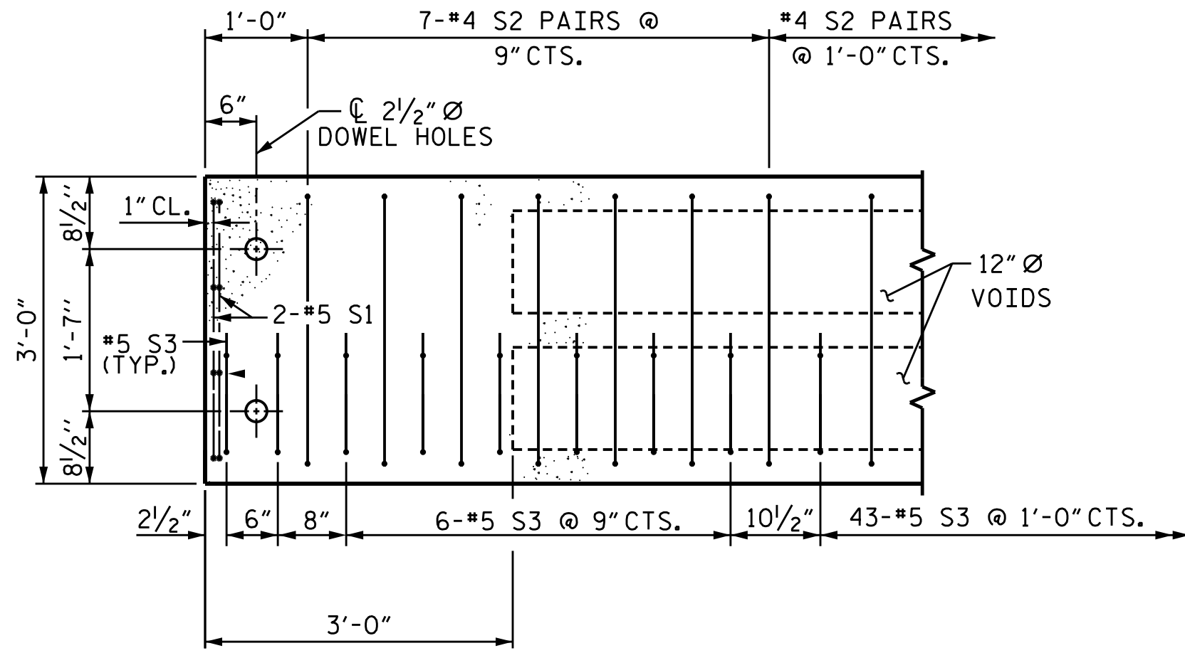
DETAIL "A"
