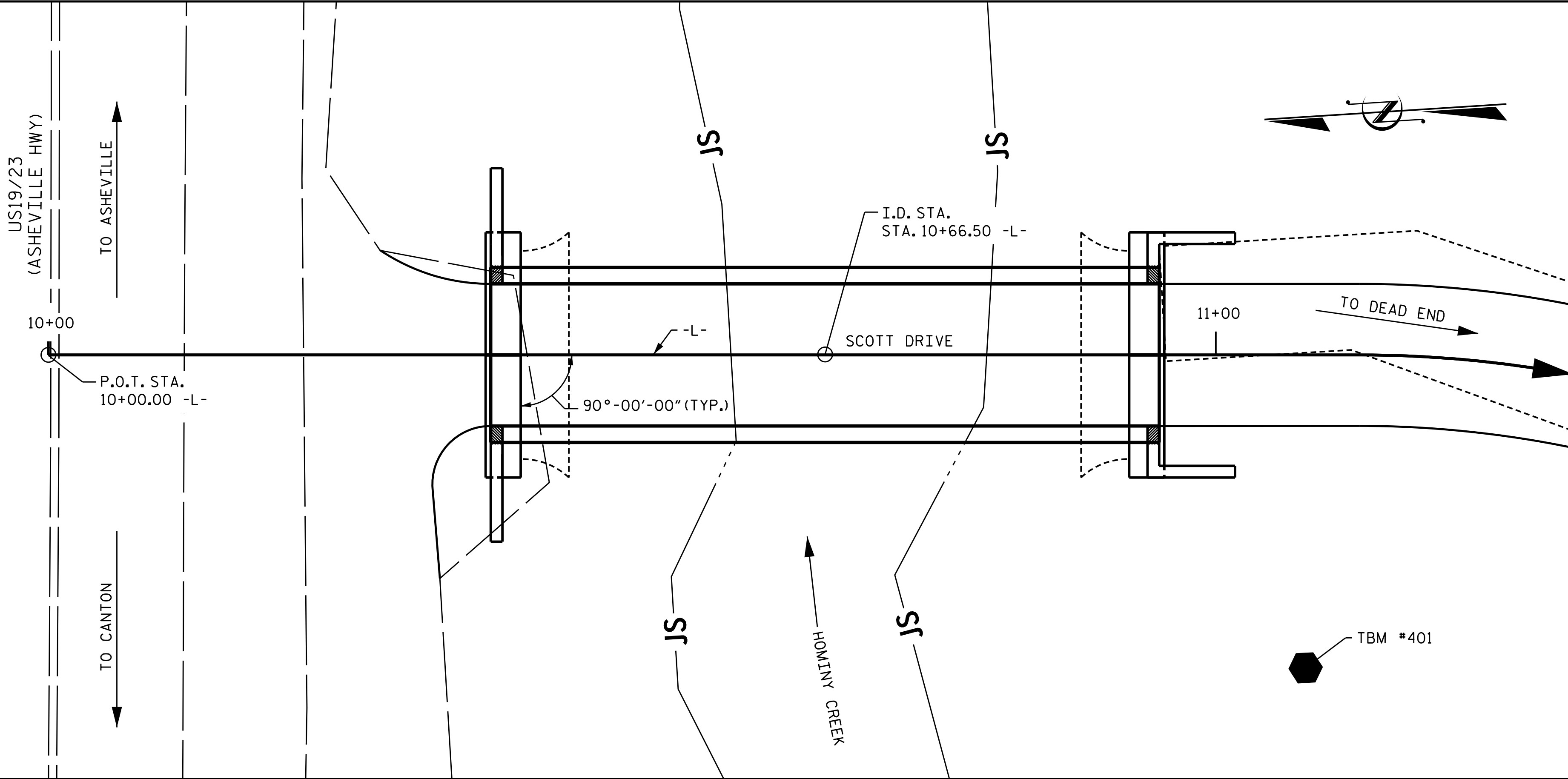
LOCATION SKETCH
