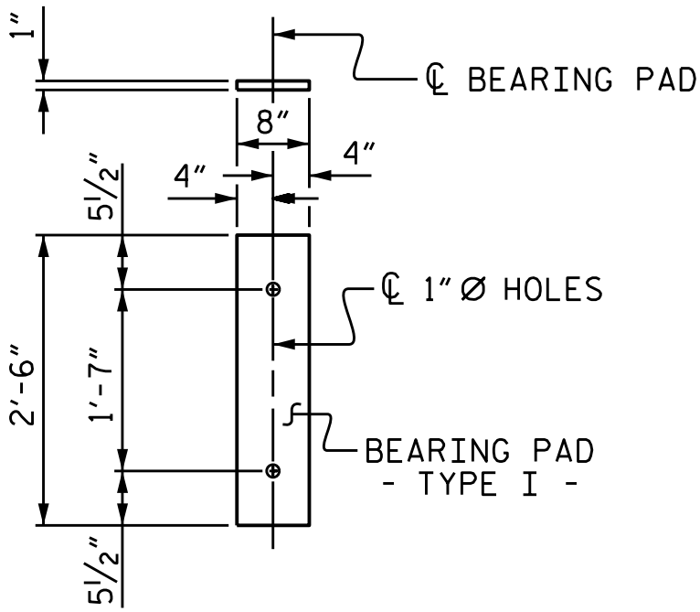
FIXED END ( TYPE I - 10 REQ'D )
