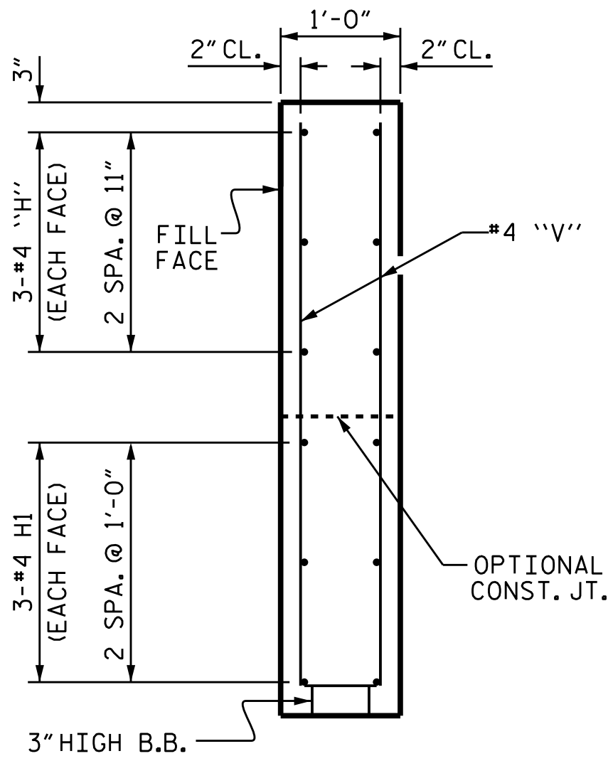
SECTION Y-Y
