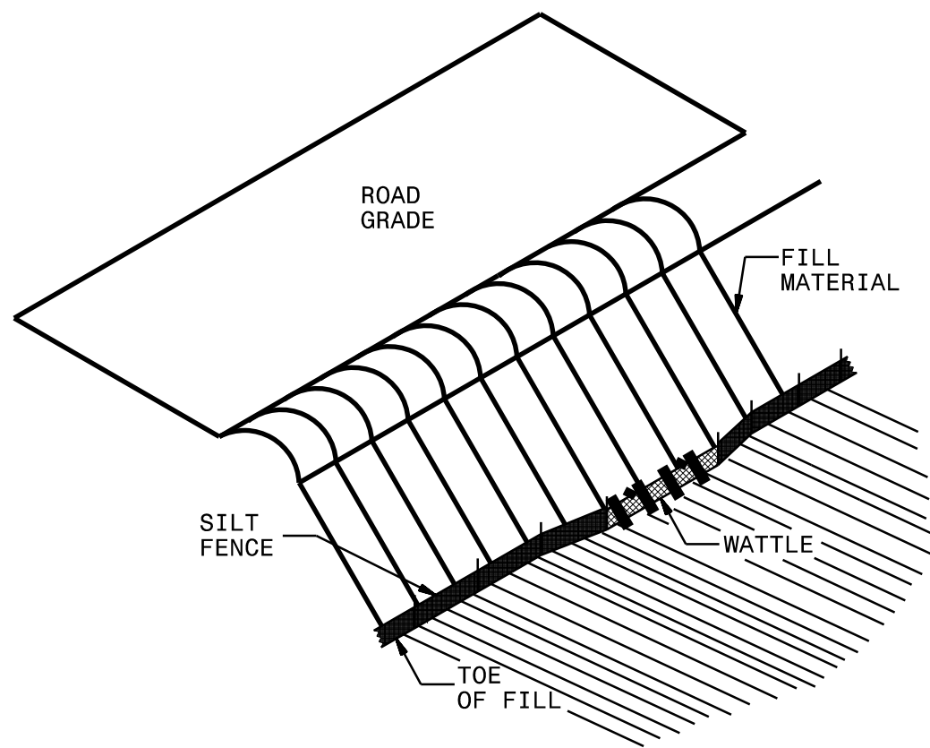
ISOMETRIC VIEW
