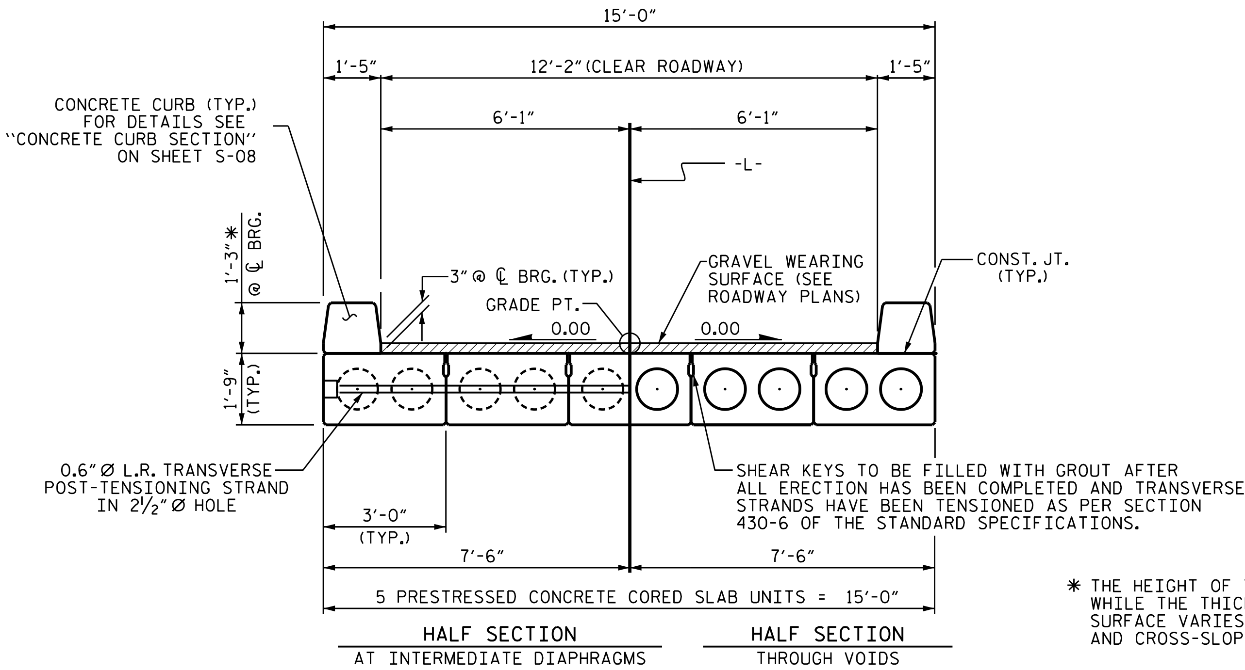
TYPICAL SECTION
