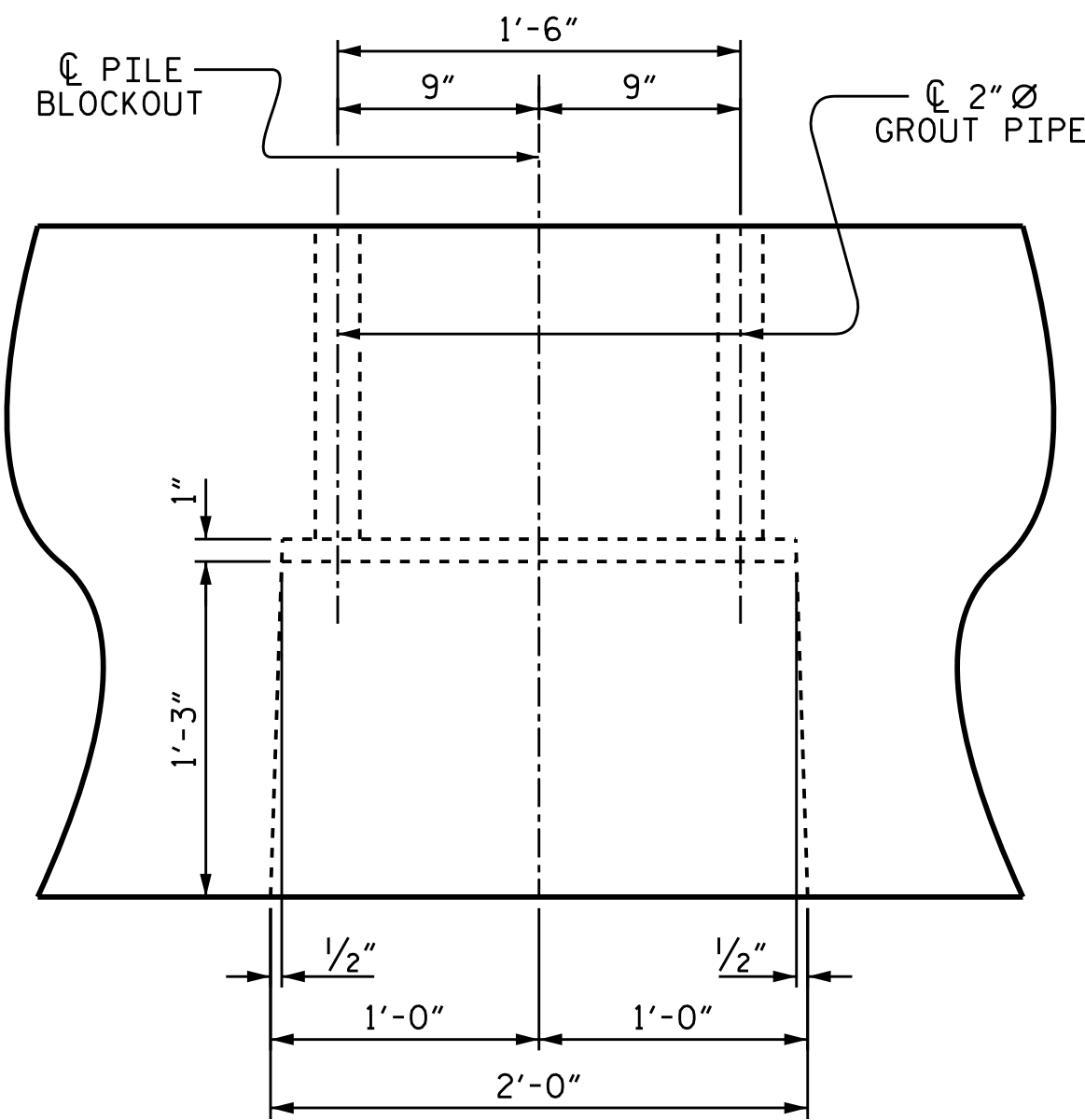
PILE BLOCKOUT DETAILS (DIMENSIONS ARE TYPICAL EACH BLOCKOUT)
