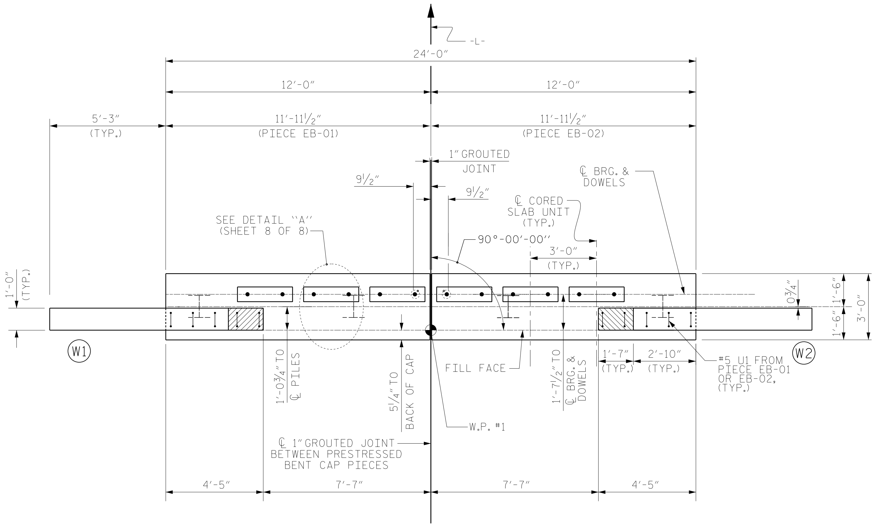
PLAN
