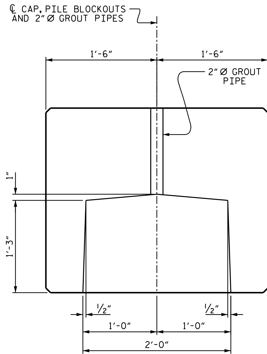
PILE BLOCKOUT DETAILS (DIMENSIONS ARE TYPICAL EACH BLOCKOUT)
